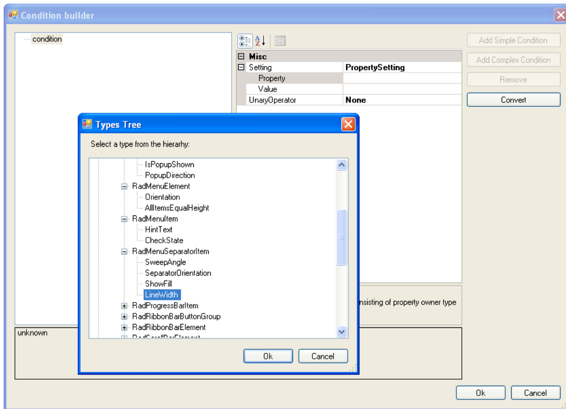
Figure 10. The Condition Builder.
