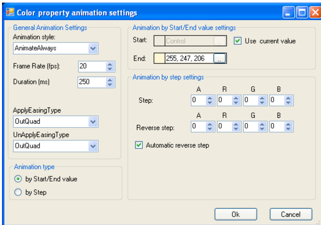
Figure 11. Setting animation properties for a color property.
