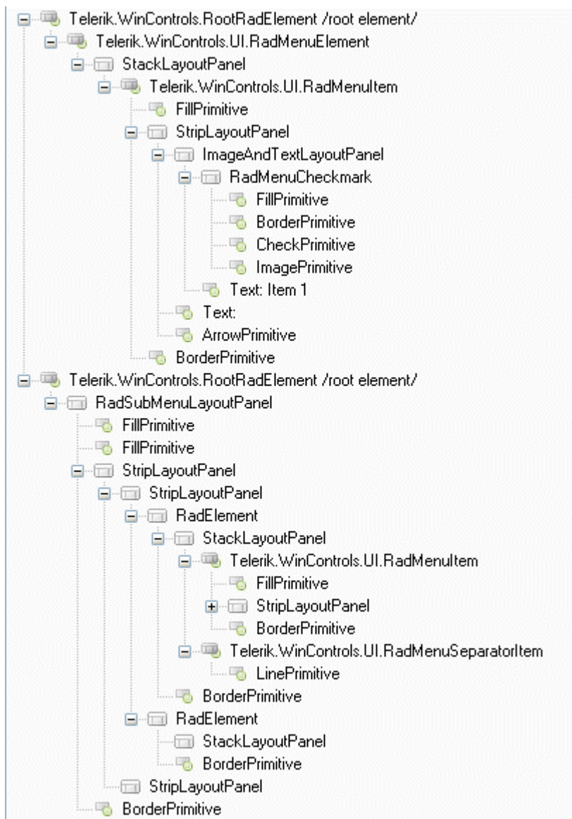
Figure 8. The elements of a RadMenuStrip.
